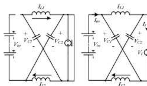
Fig. 1 Topology with bidirectional ZSI for PMSM drive
