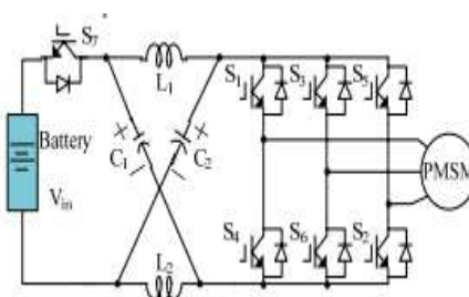
Fig. 1 Topology with bidirectional ZSI for PMSM drive
