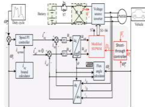
Fig.3 Control scheme of PMSM drive system with ZSI for EV
