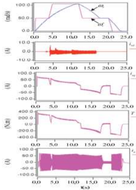
Fig. 5. Transient waveforms for PMSM driven by ZSI
