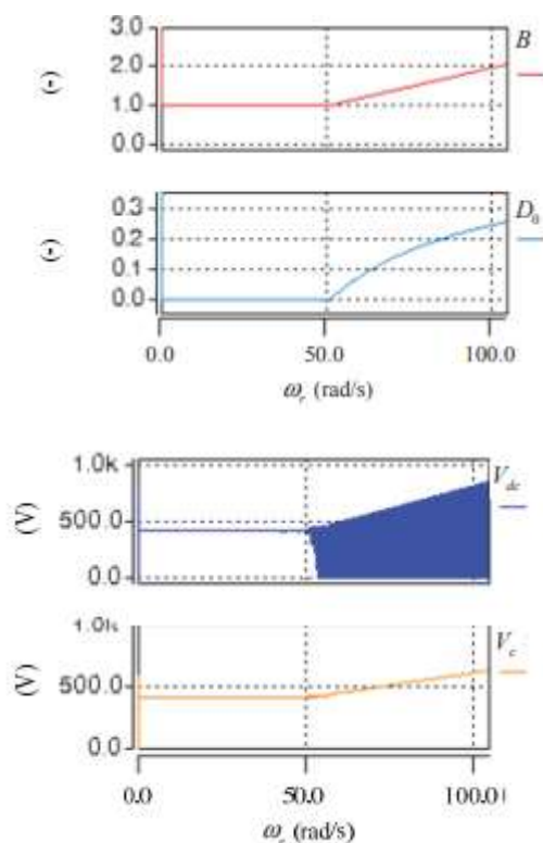
Fig. 7 (a) Boost factor and shoot-through time duty ratio versus speed characteristics (b) DC-link voltage and capacitor voltage versus speed characteristics F per loss by the current is generated.
